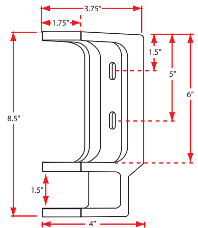
L series Dual-use Bracket
